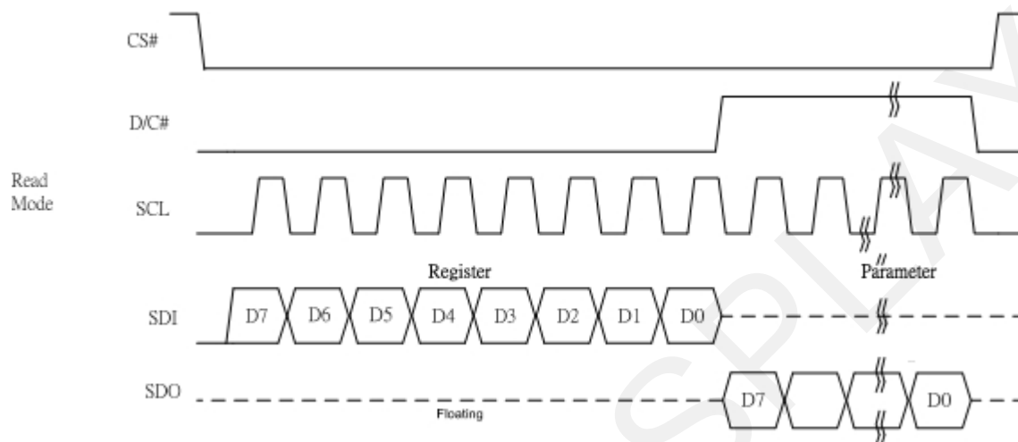
Figure 3.5-1: wire mode
